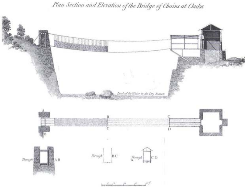
Fig. 39: The drawing of the Chukha Chaksam published by Samuel Turner in 1800 in London after the exact measurement of his travel companion Samuel Davis. Source: Turner, 1800
